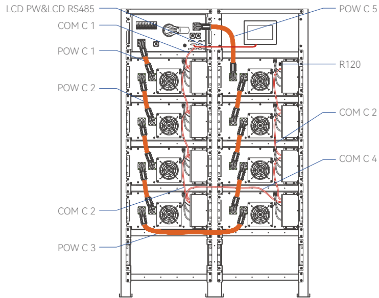
Wiring diagram
