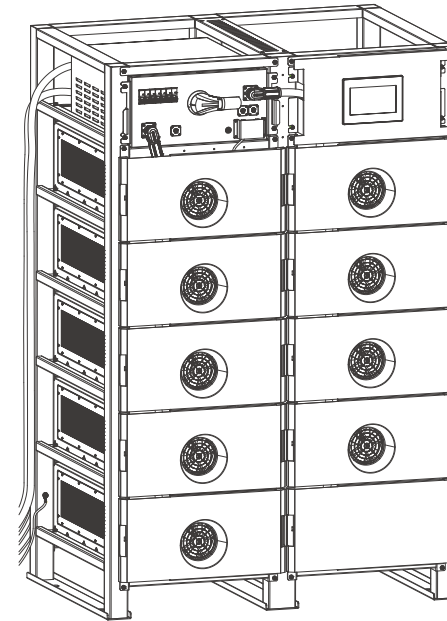
Figure 2.19 Overall diagram
