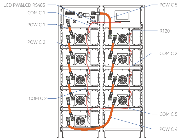
Wiring diagram
