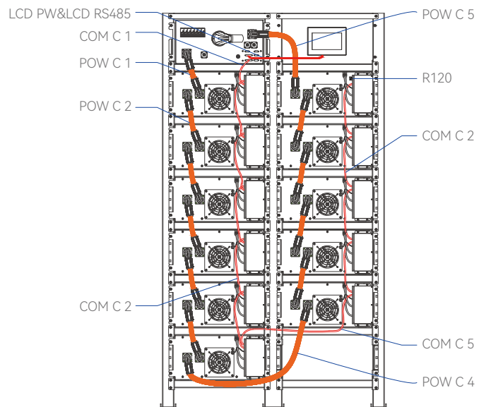
Wiring diagram
