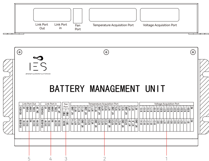
Figure 2.4 BMU photo
