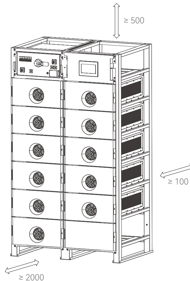
Figure 1.1 Schematic diagram of reserved space
