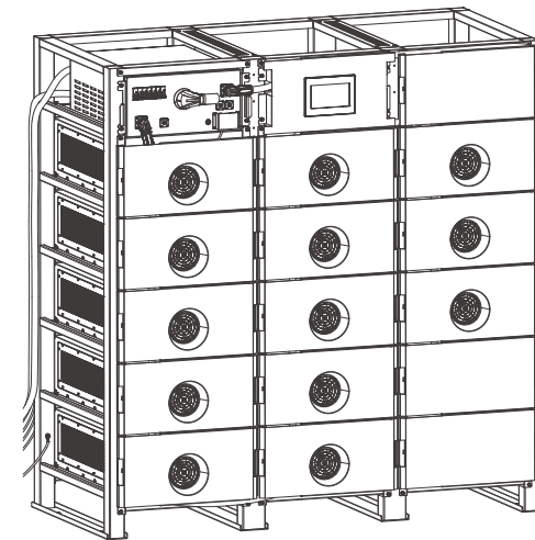
Figure 2.21 Overall diagram
