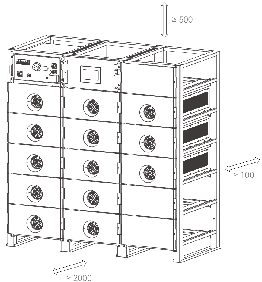
Figure 1.1 Schematic diagram of reserved space
