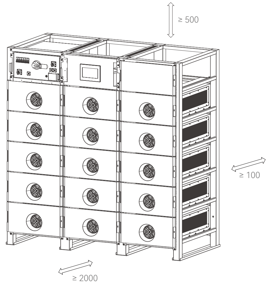
Figure 1.1 Schematic diagram of reserved space
