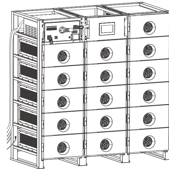
Figure 2.21 Overall diagram
