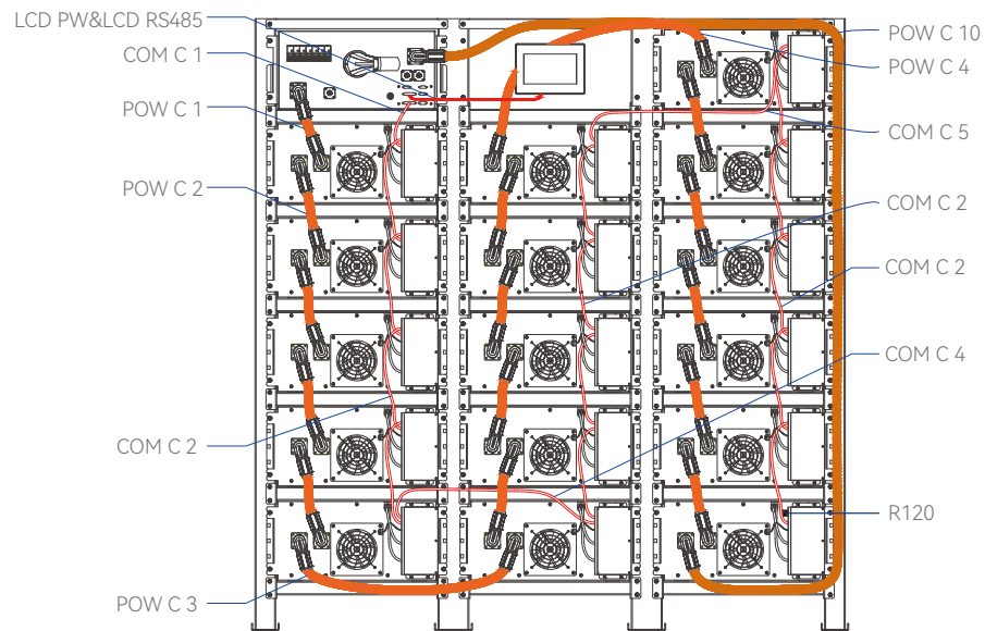
Wiring diagram
